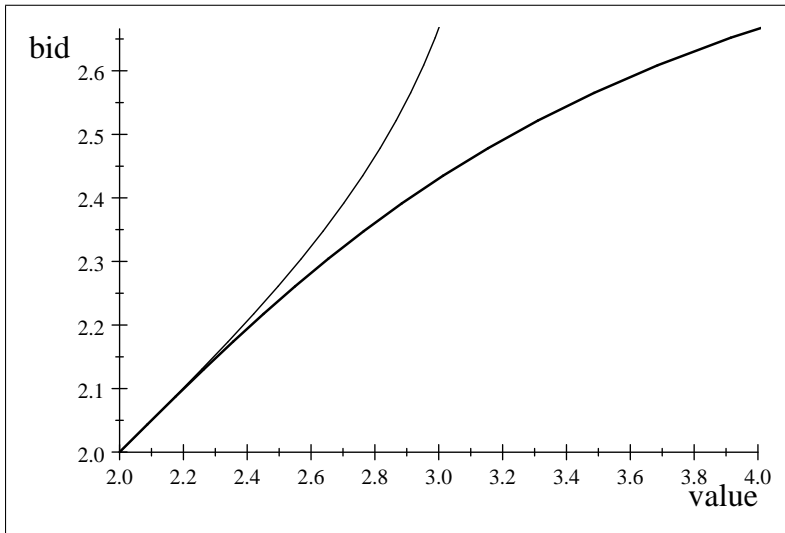
Figure 2: Solution to modified Example 1 when v_1 = 2, v_2 = 2, \bar{v}_2 = 3, \bar{v}_1 = 4 . The thicker line is v_1(b) .
