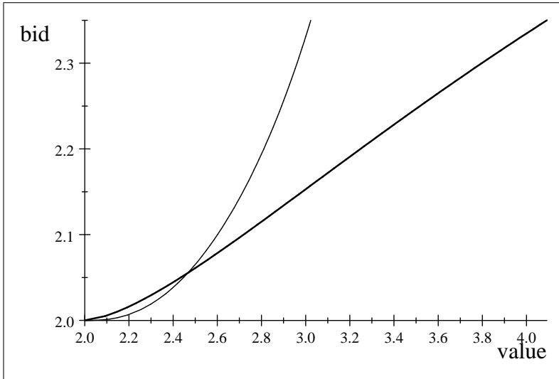
Figure 1: Solution to Example 1, v_1 = 0 , v_2 = 1 , m = 2 , \bar{v}_2 = 3 , \bar{v}_1 = 4 . The thick line is v_1(b) .
